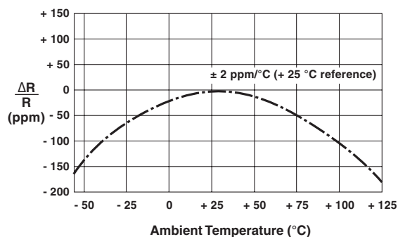
FIGURE 4 - TYPICAL TCR CURVE
